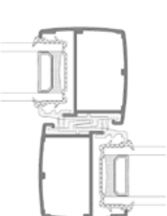
Interlock Detail
