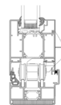
Cill Detail
