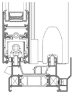
Cill Detail
