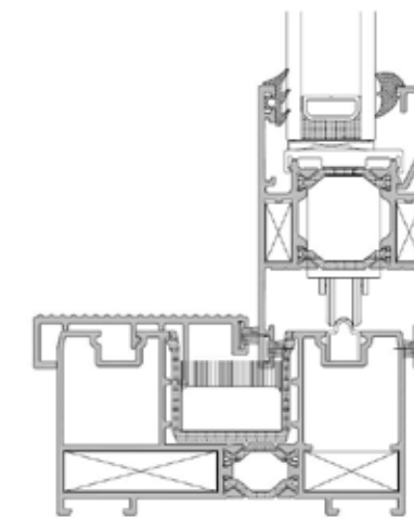
Cill detail
