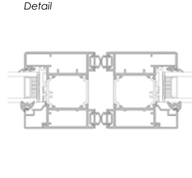
Leaf-Leaf Detail
